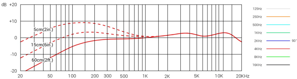
Frequency Response
