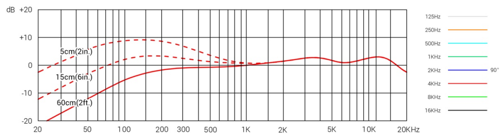
Frequenzgang
