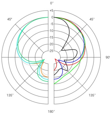
Polar Pattern
