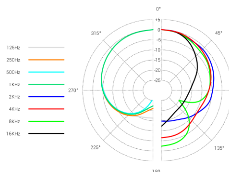
Polar Pattern
